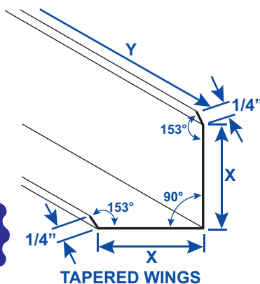
TAPERED WINGS
